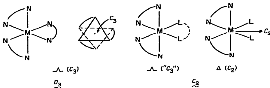
Fig 5 "Configuration relationship" behavior between \text{Co}(\text{en})_3^{3+} and \text{Co}(\text{en})_2\text{L}_2^{n+}
