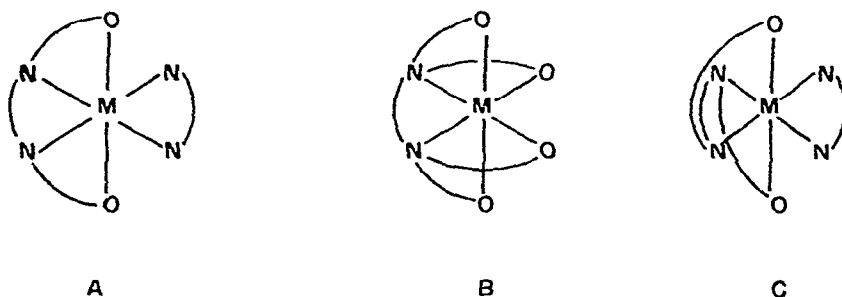
Fig 8. Configurational comparison between \text{s-cis-[Co(EDDA)(en)]}^+ and [\text{Co(EDTA)}]^-
